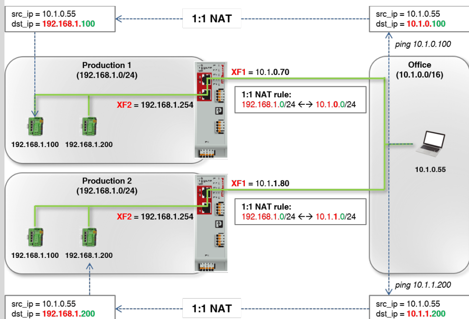
Figure 6-10 Example: 1:1 NAT (identical networks)
