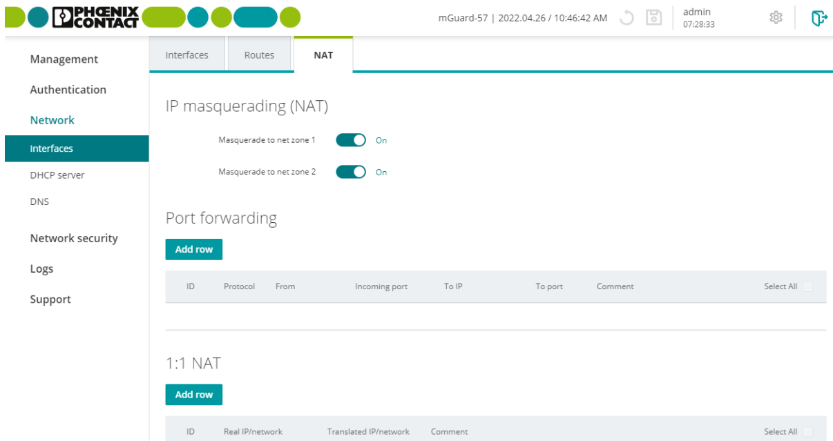
Figure 6-6 Network >> Interfaces >> NAT: IP masquerading, port forwarding, and 1:1-NAT configuration
