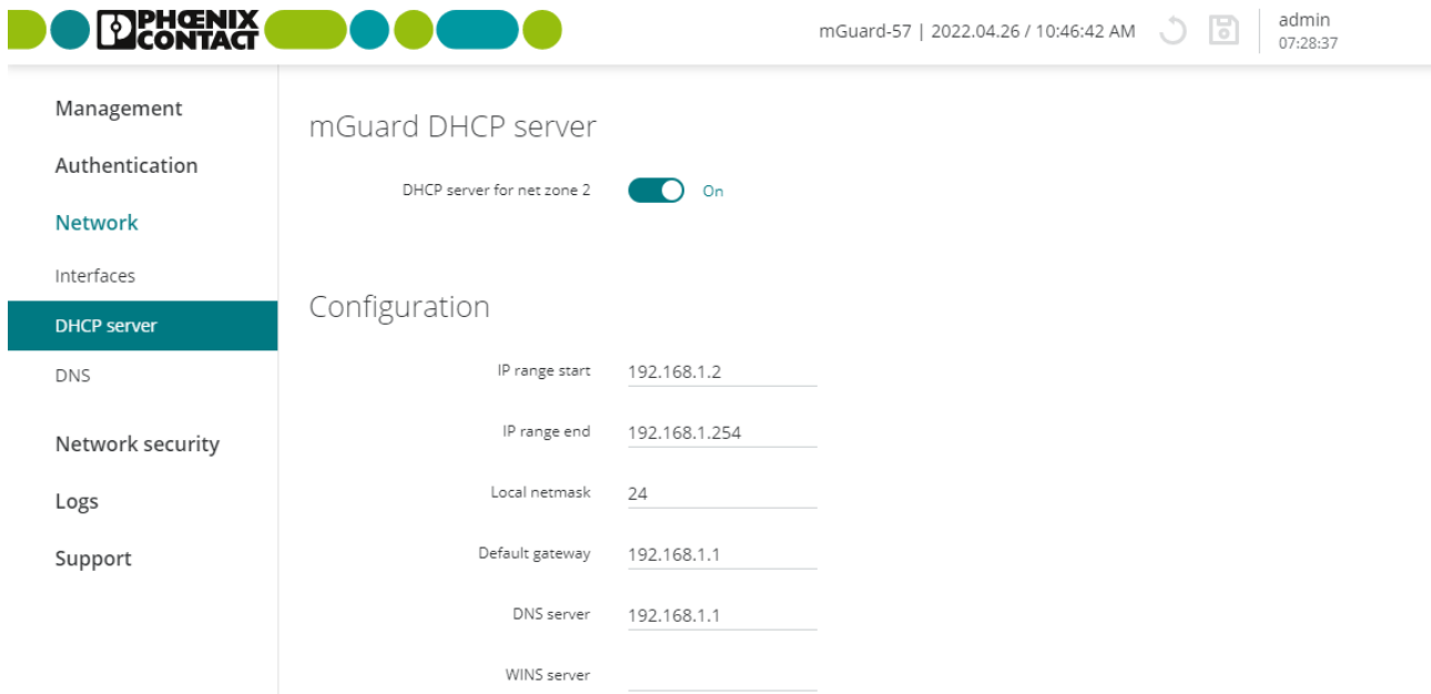
Figure 6-11 Network >> DHCP server: Configure DHCP server
