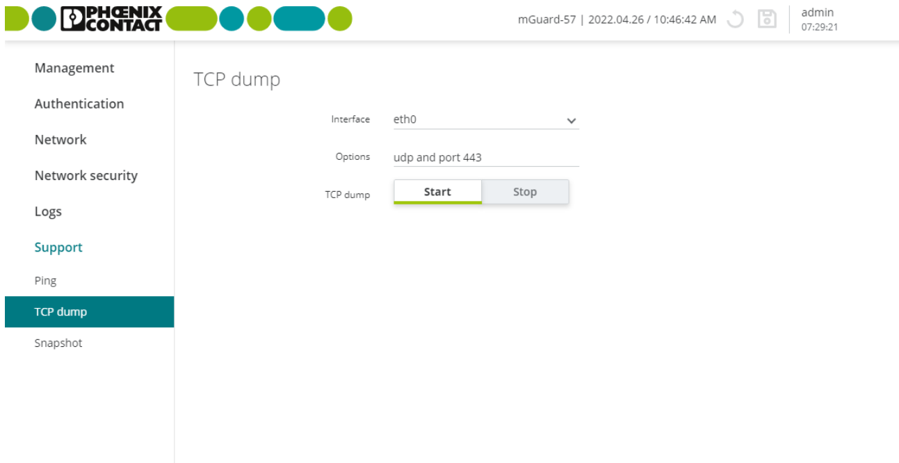
Figure 9-2 Support >> TCP dump
