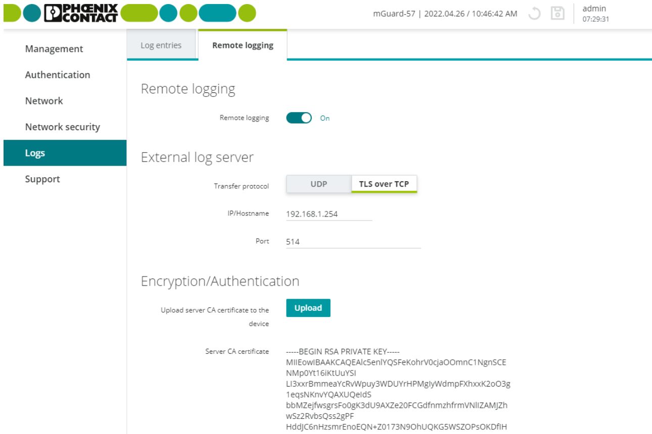
Figure 8-2 Logging >> Remote logging (syslog)
