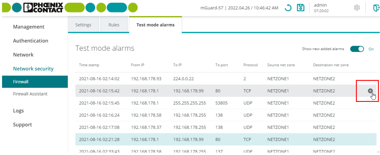
Figure 7-3 Network security >> Firewall >> Test mode alarms
