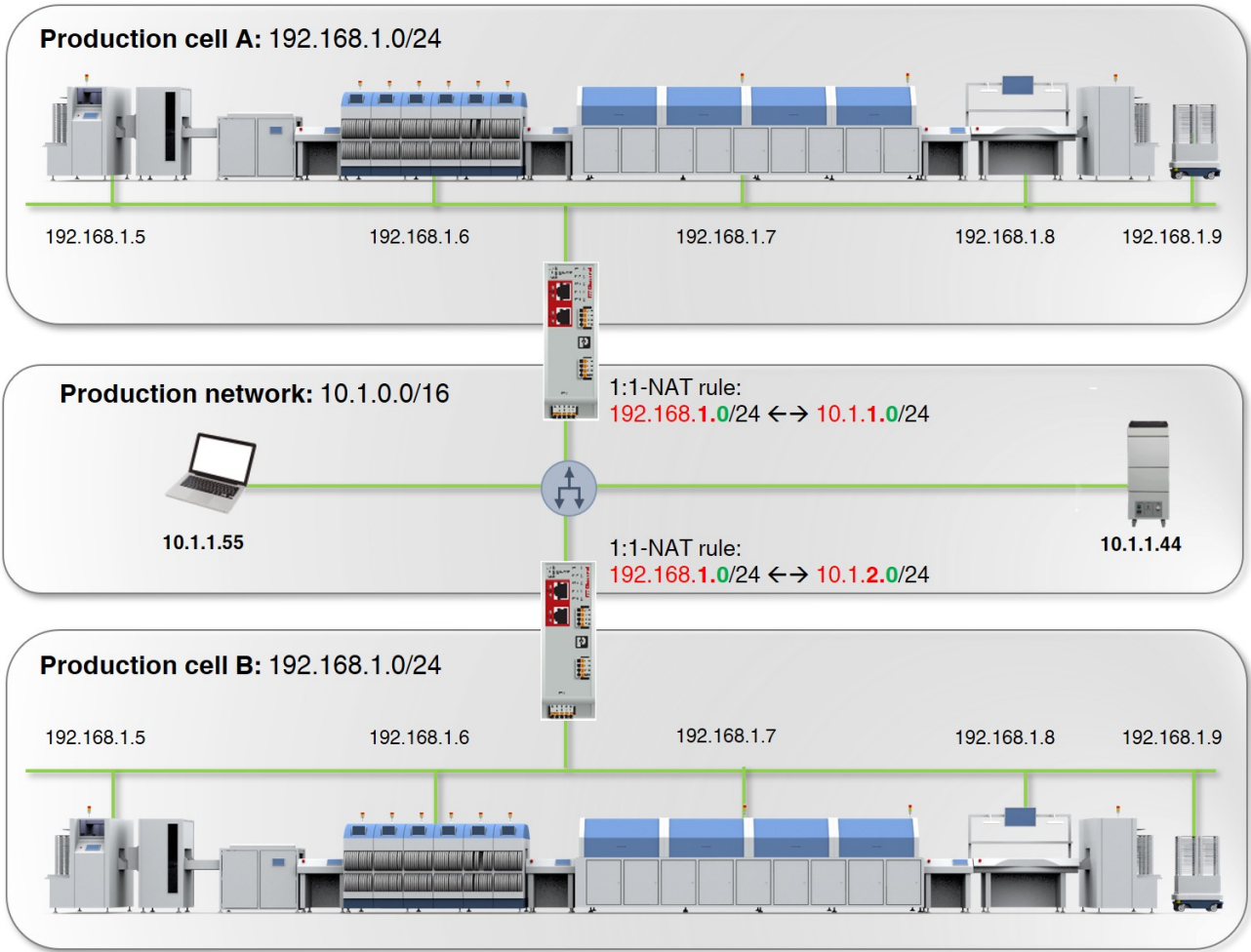
Figure 2-1 Using the device as a NAT router (example: 1:1 NAT)
