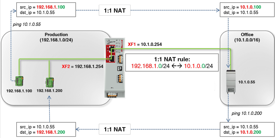
Figure 6-9 Example: 1:1 NAT (two networks)
