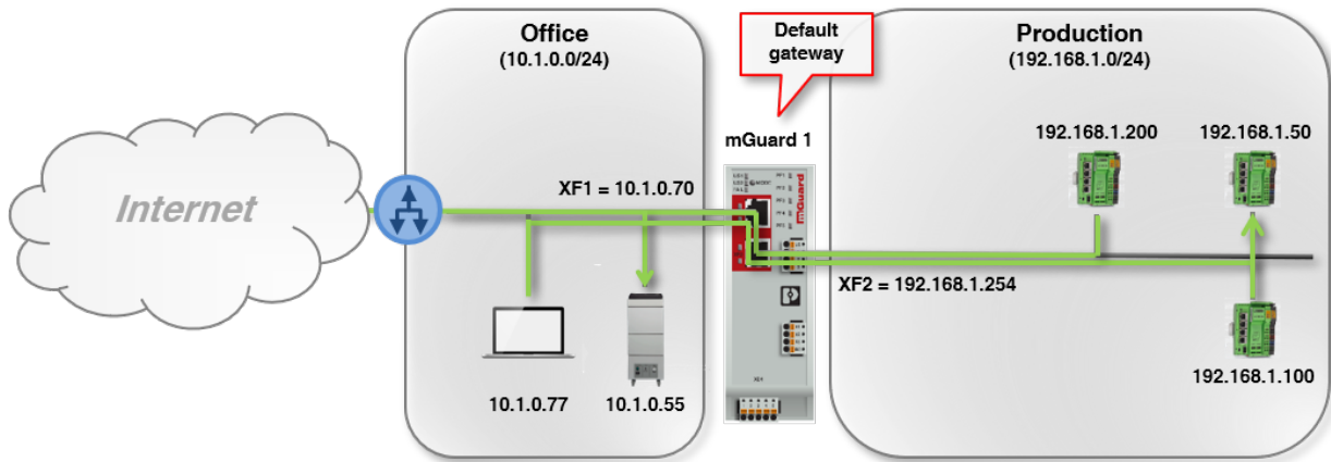
Figure 6-2 Example: Router mode
