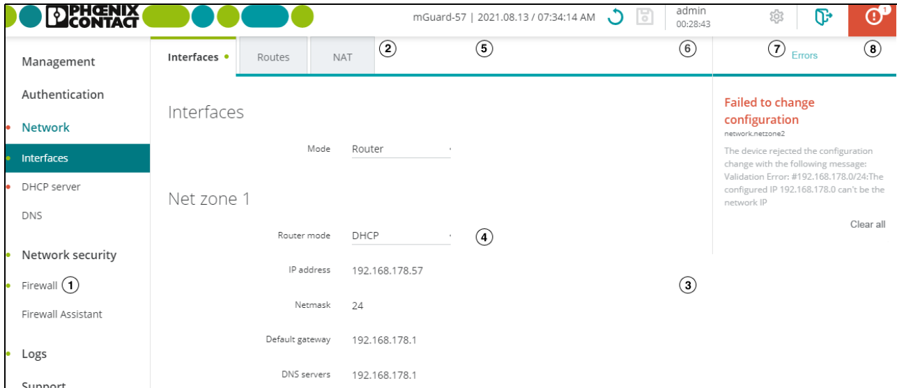
Figure 3-4 Web-based management: Menu structure and page elements
