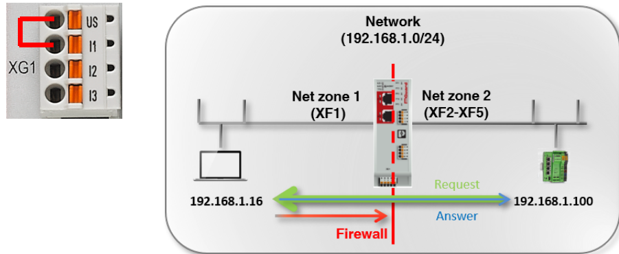
Figure 2-2 Activated Easy Protect Mode (via cable bridge)
