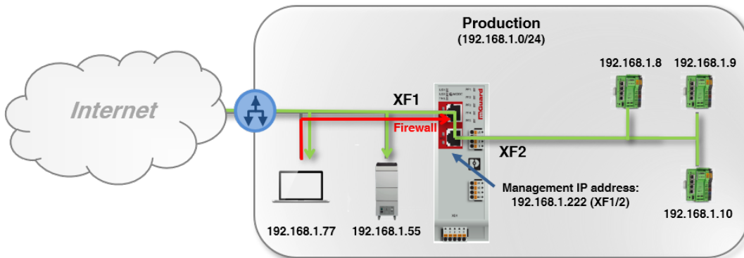
Figure 6-3 Example: Stealth mode (with activated firewall XF1 --> XF2)
