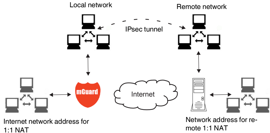
Figure 10-3 1:1 NAT
