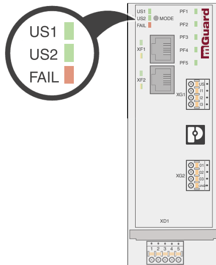
Figure 3-7 LEDs: US1 and US2
