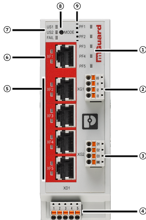
Figure 3-3 FL MGUARD 2105: Operating elements and LEDs
