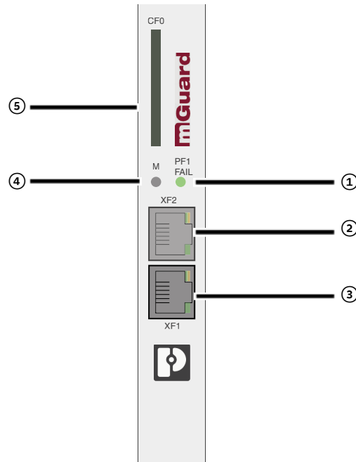
Figure 4-2 FL MGUARD 4102 PCI(E): Operating elements and LEDs
