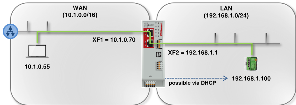
Figure 5-1 Operating the device in router mode (example configuration)
