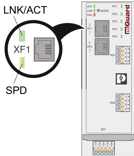
Figure 3-6 LED: LNK/ACT and SPD
