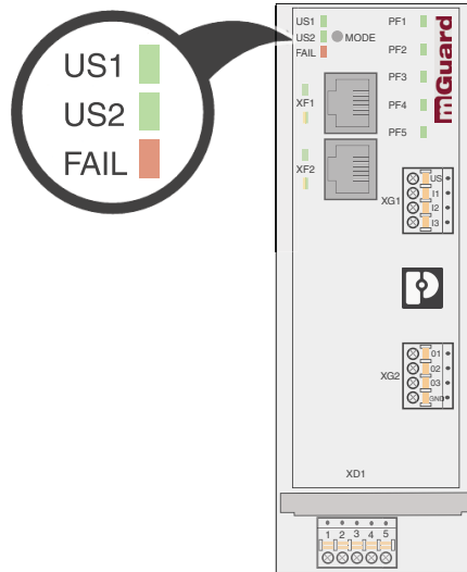
Figure 3-8 LED: FAIL
