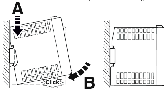
Figure 3-9 Snapping the device onto a DIN rail
