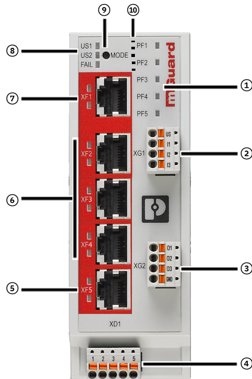
Figure 3-4 FL MGUARD 2102/FL MGUARD 4302: Operating elements and LEDs
