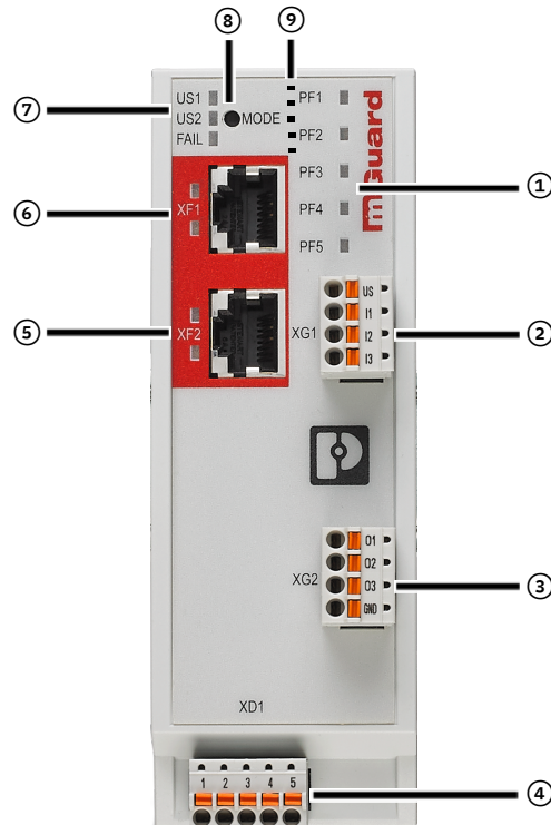
Figure 3-2 FL MGUARD 2102/FL MGUARD 4302: Operating elements and LEDs
