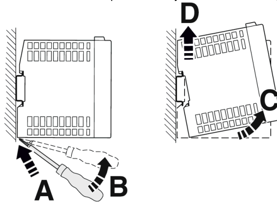
Figure 3-10 Removing the device
