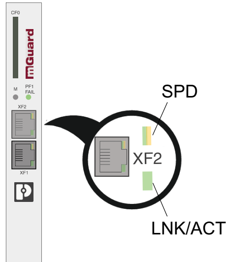
Figure 4-3 LEDs: SPD and LNK/ACT
